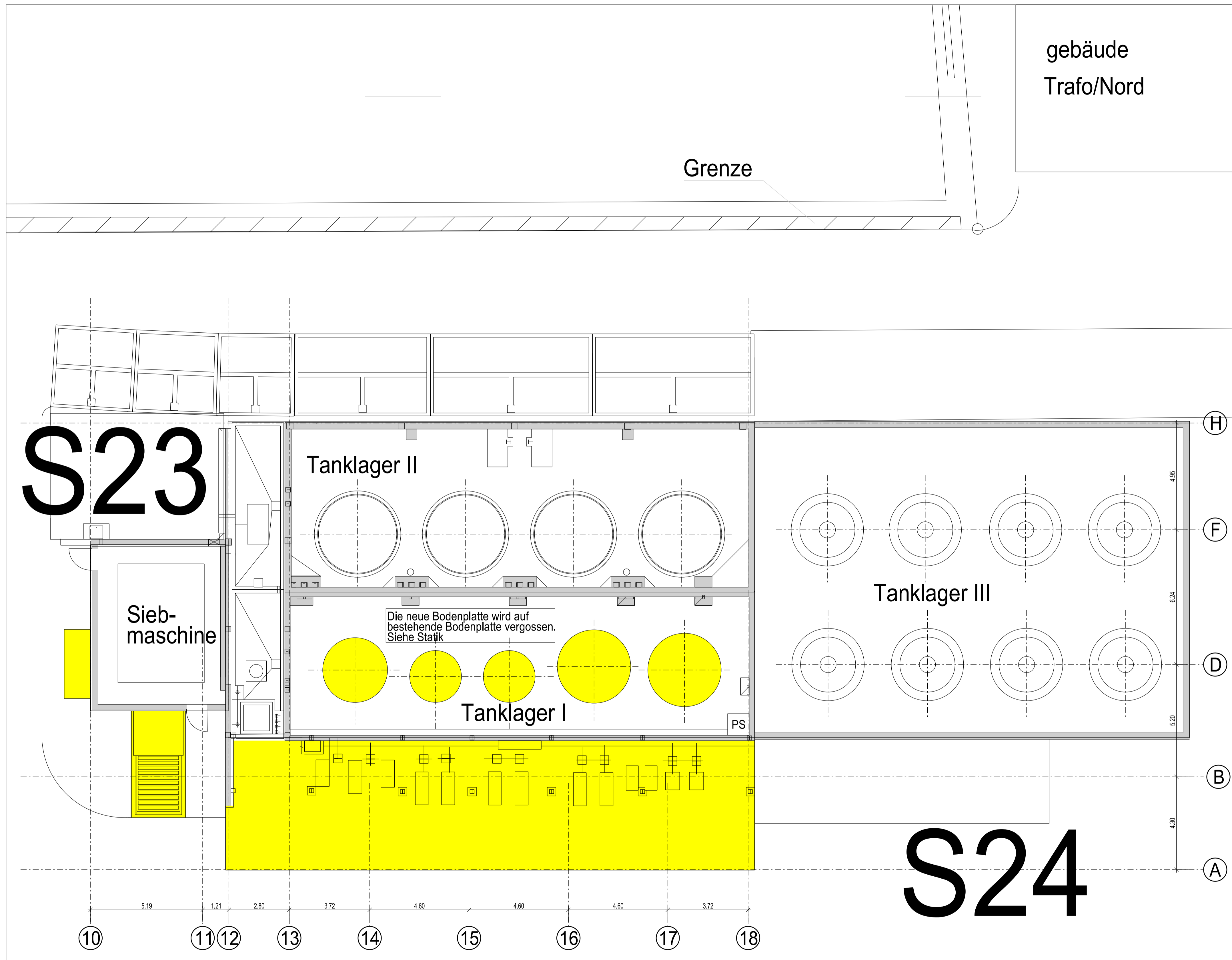
Grundriss ±0.00m
